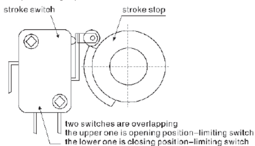
drawing 3
