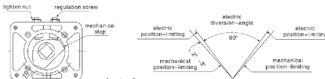
drawing 5
